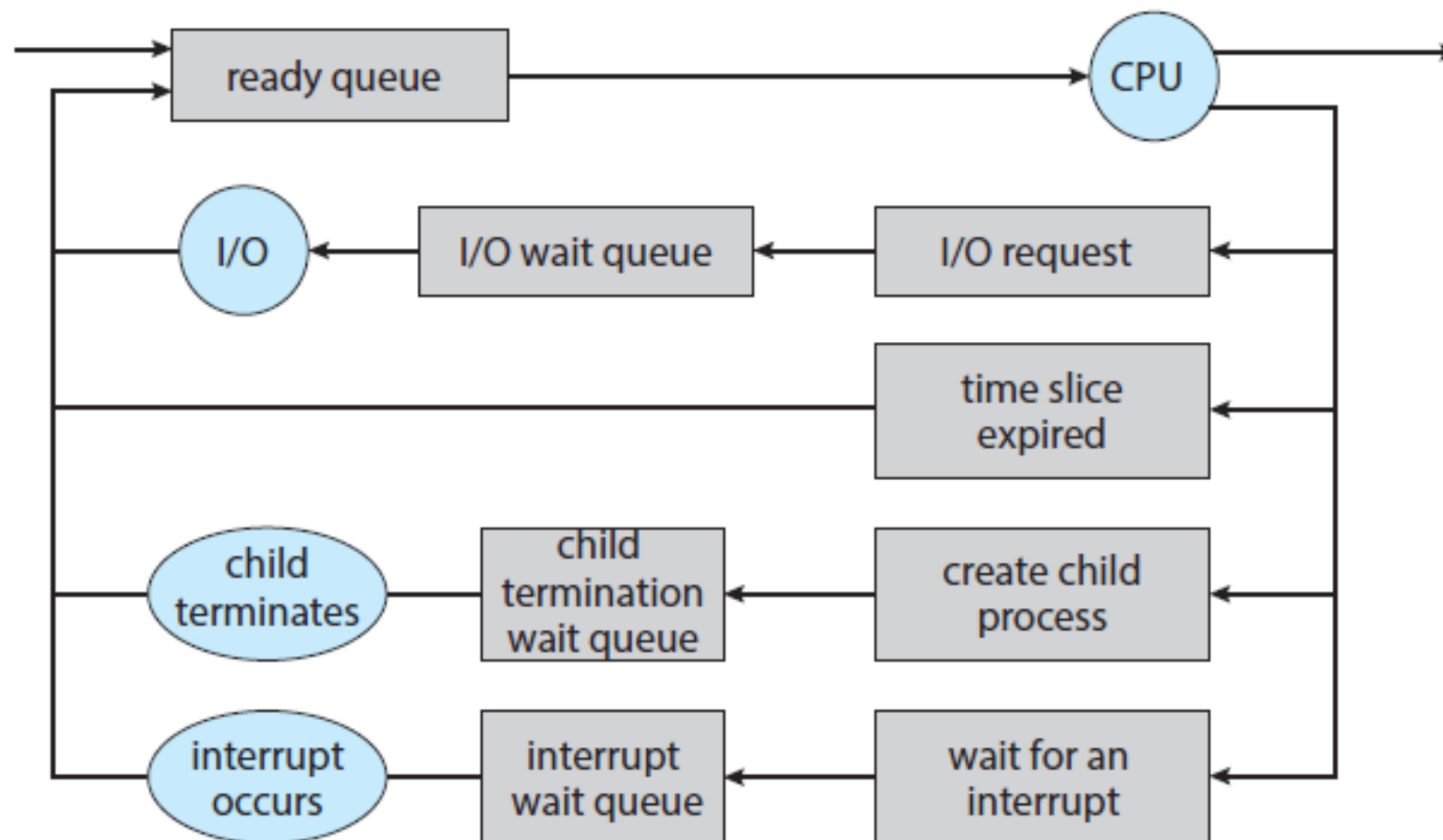
Figure: Queuing-diagram representation of process scheduling.
