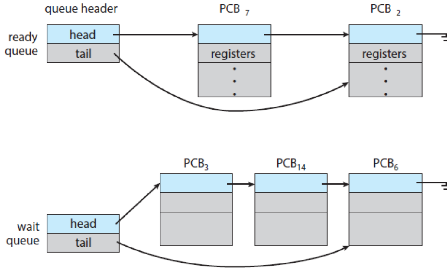
Figure: The ready queue and wait queues.
